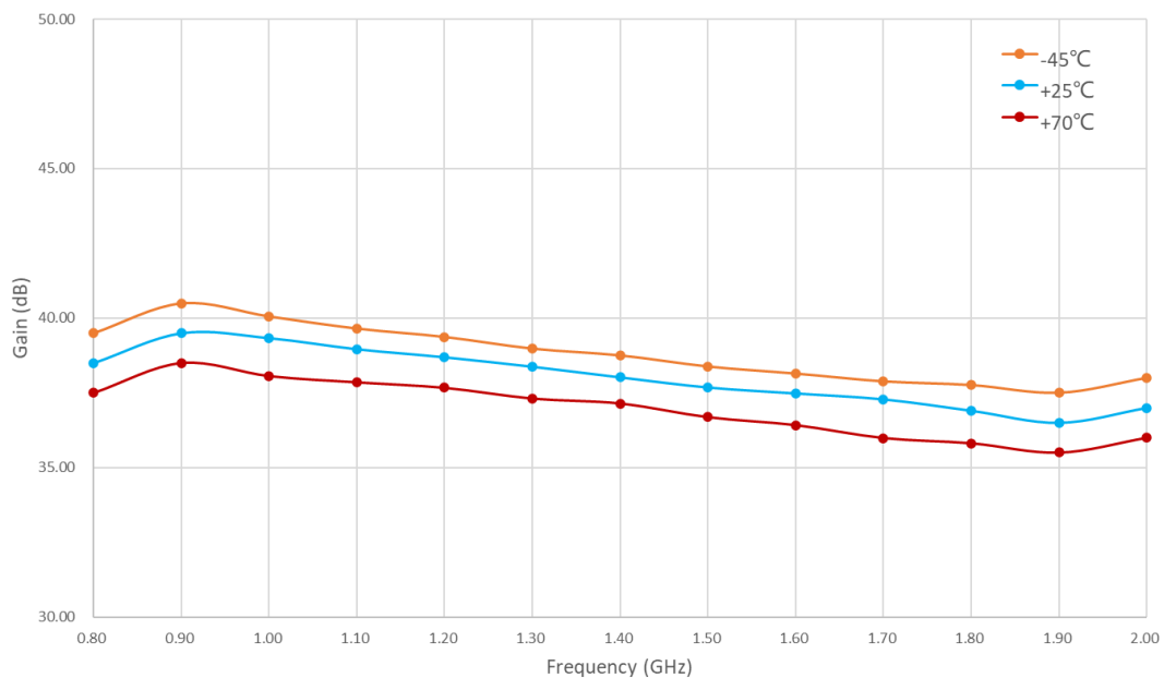
Figure 2: GPA-0080-0200-50 Small Signal Gain Vs Temperature
