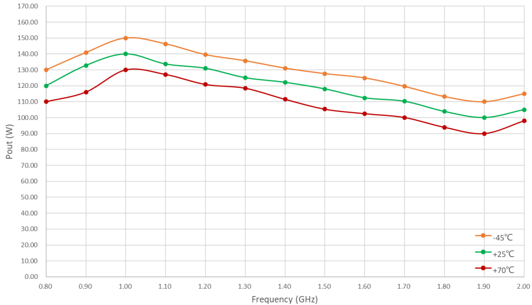
Figure 1: GPA-0080-0200-50 Psat
