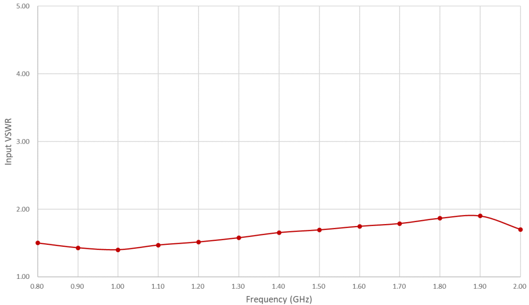
Figure 3: GPA-0080-0200-50 Input VSWR
