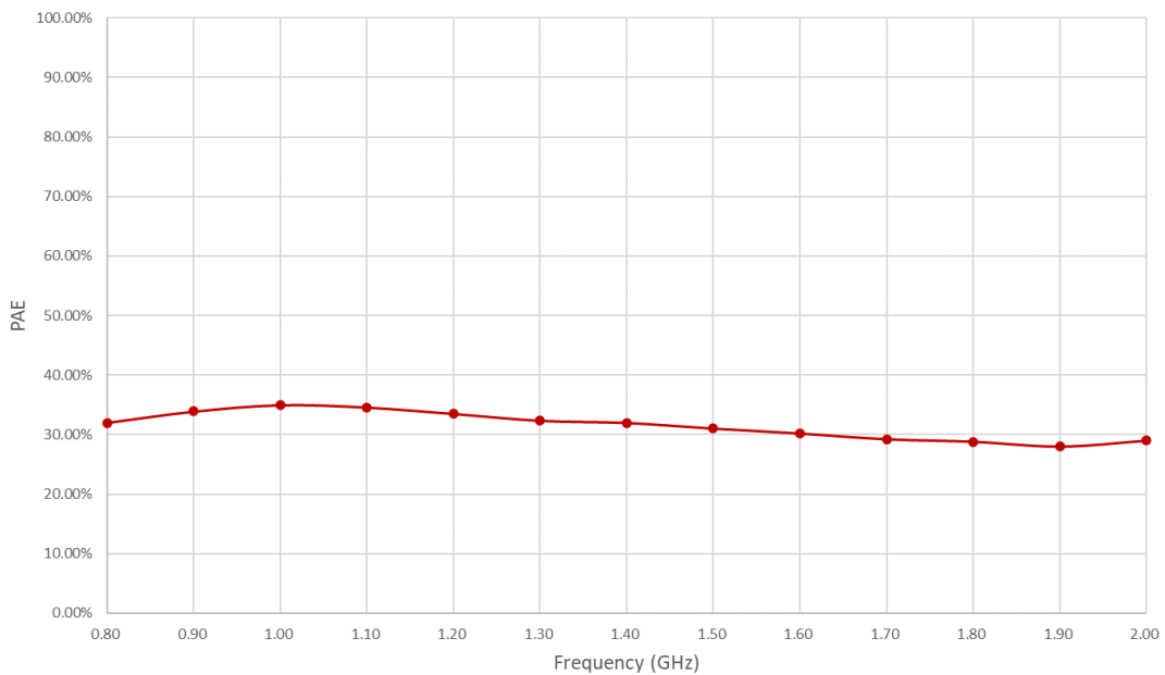
Figure 4: GPA-0080-0200-50 P.A.E
