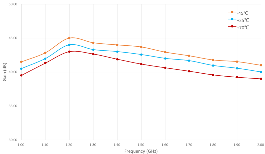
Figure 2: PPA-0100-0200-50 Small Signal Gain Vs Temperature
