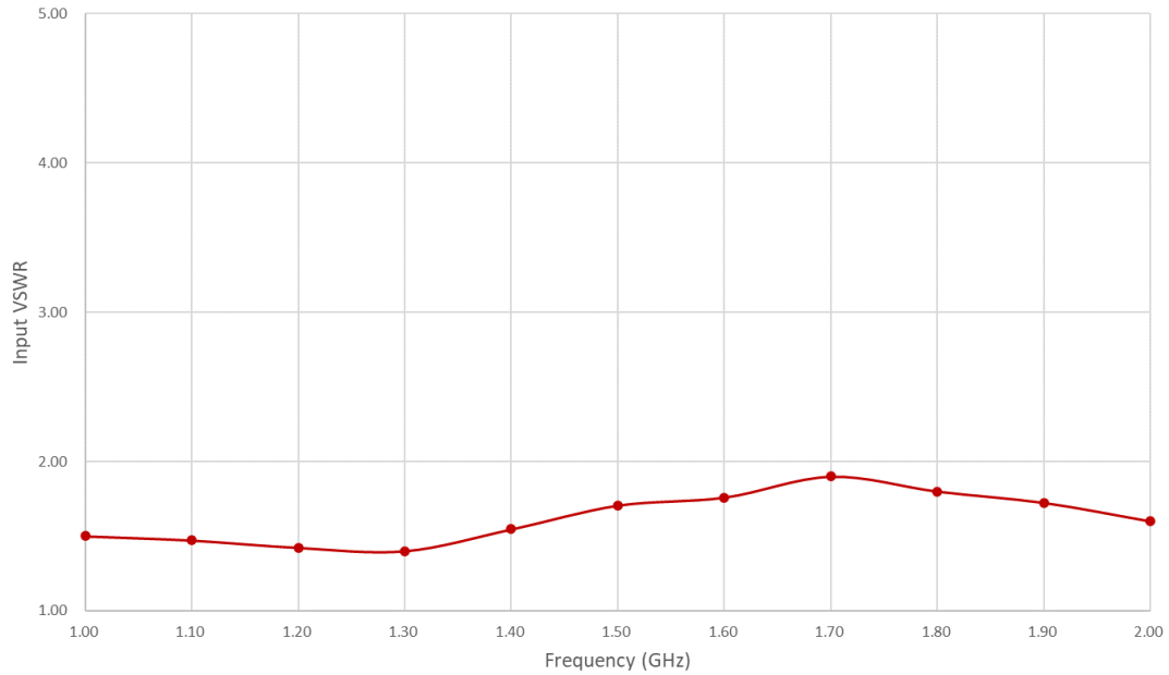
Figure 3: PPA-0100-0200-50 Input VSWR
