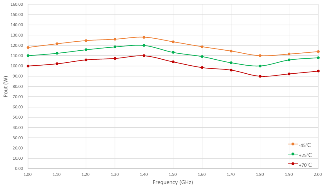
Figure 1: PPA-0100-0200-50 Psat
