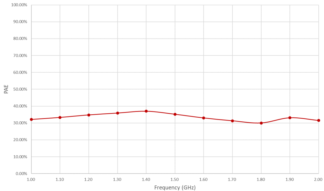
Figure 4: PPA-0100-0200-50 P.A.E
